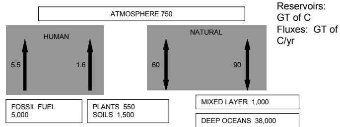
The Carbon Cycle, from IPCC (1995)
