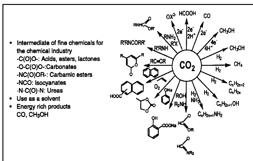
Figure 1 Utilization of Carbon Dioxide in Synthetic Chemistry, from Creutz and Fujita, 2000.
